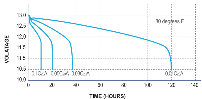
Discharge characteristics
